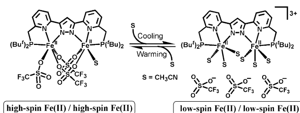
Scheme 3. Triflate/MeCN ligand exchange and spin state switching.
